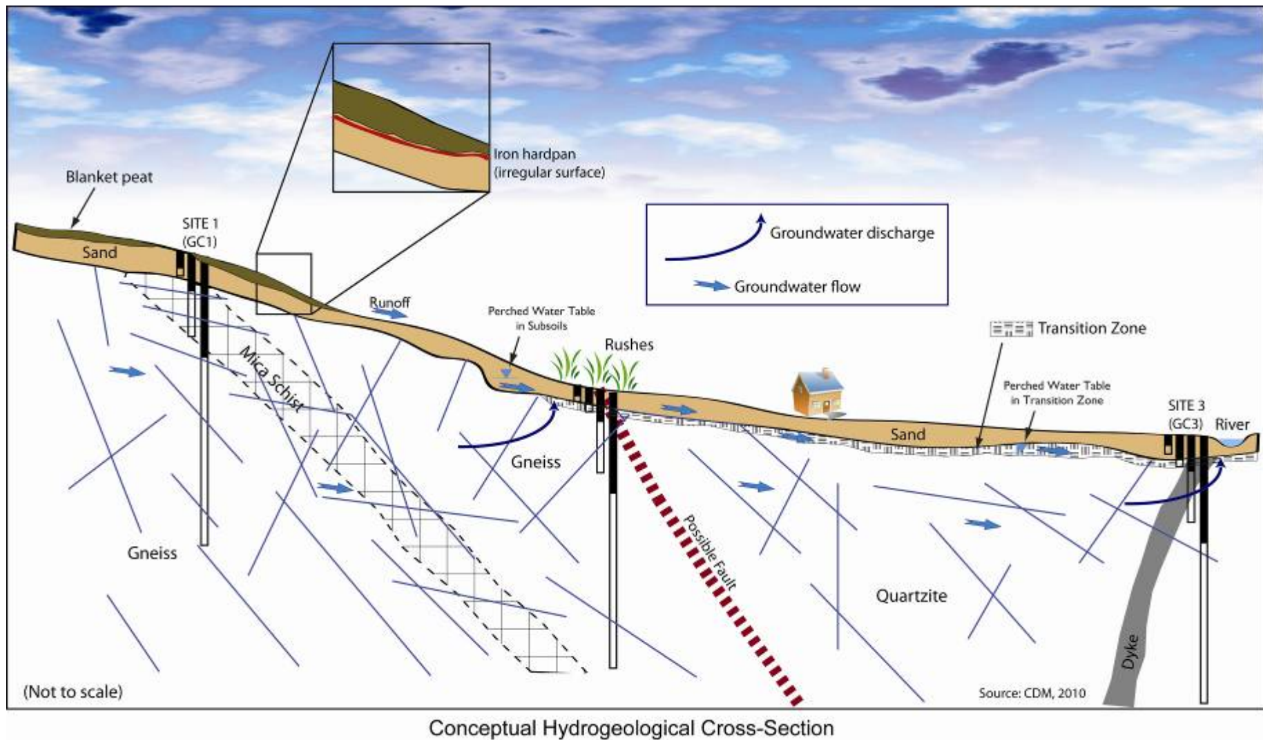
Figure G. 5 – Example of a Conceptual Hydrogeological Cross-section in a Poorly Productive Bedrock Aquifer
