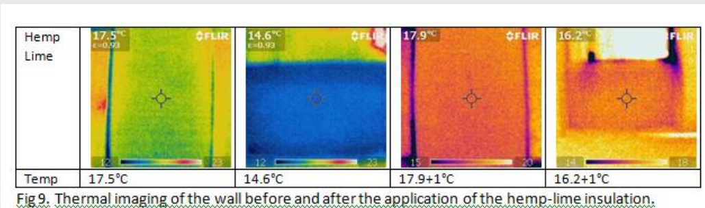
Fig 9. Thermal imaging of the wall before and after the application of the hemp-lime insulation.
