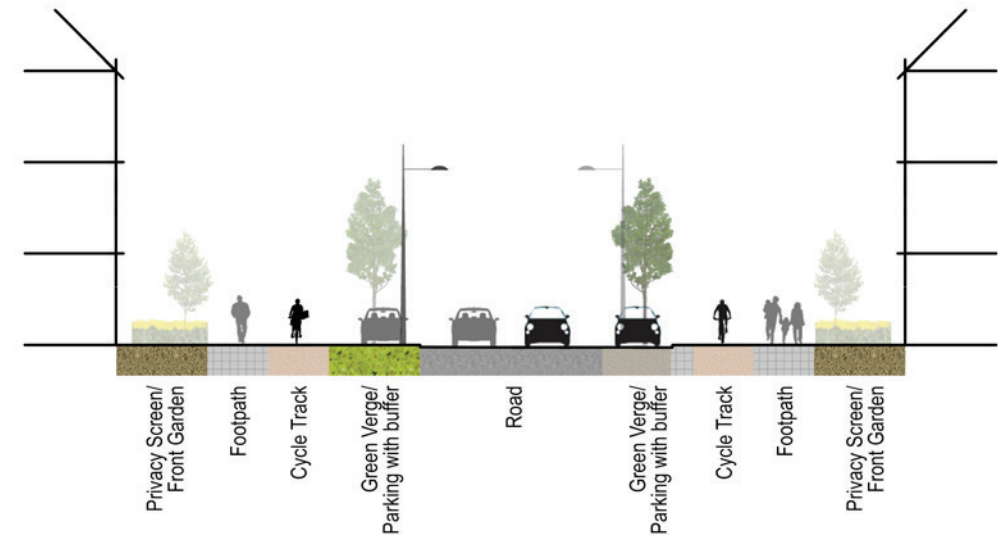
Fig. 6.9 Local Street (Medium/High Density)
