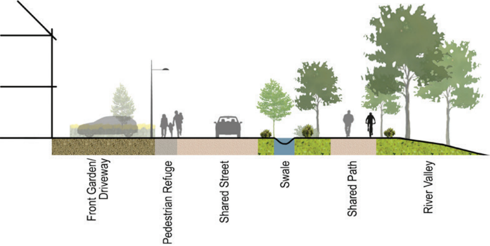
Fig. 7.3 B-B River Breaghagh Valley Interface Swale
