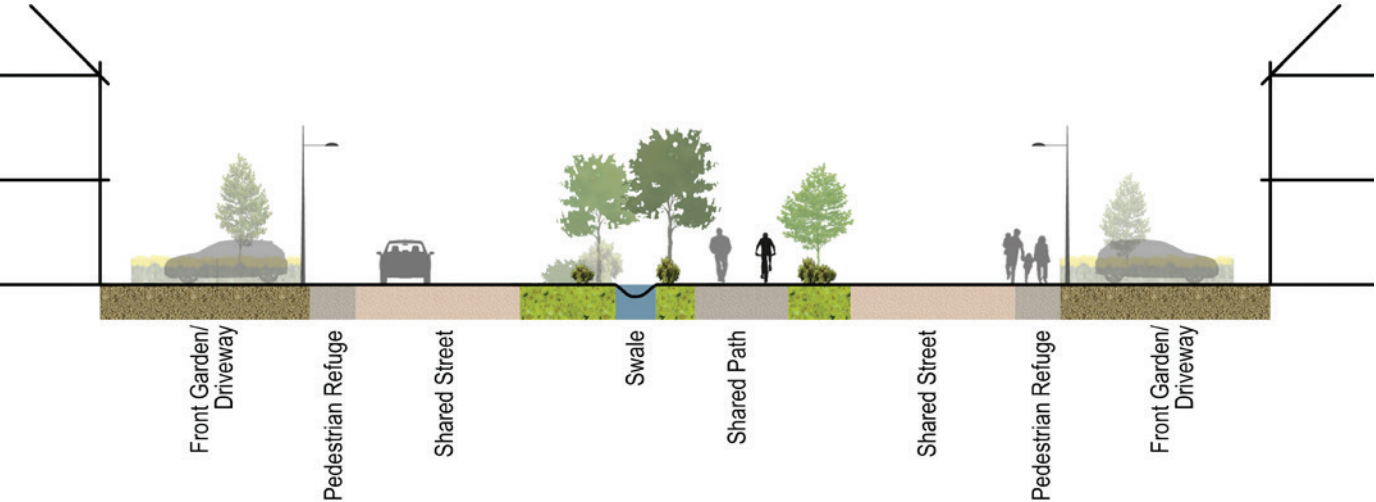
Fig. 7.2 A-A Linear Park /Green Link Swale
