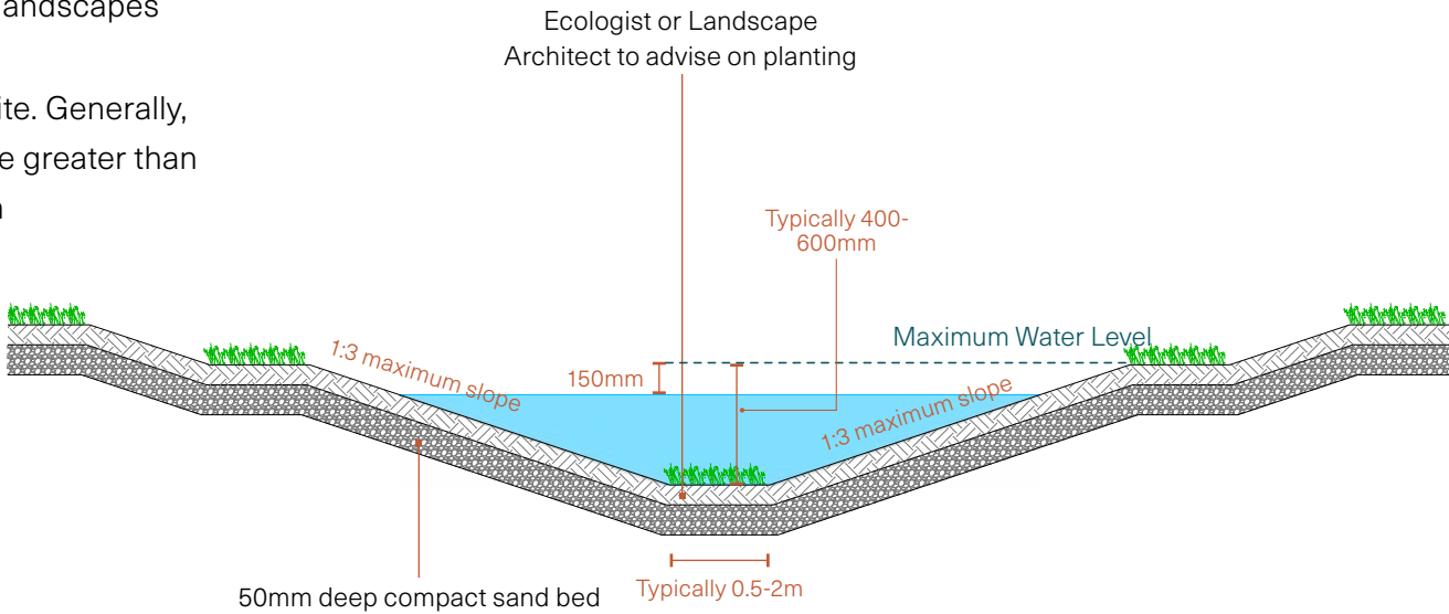
Figure 9: Typical Wet Swale Detail
