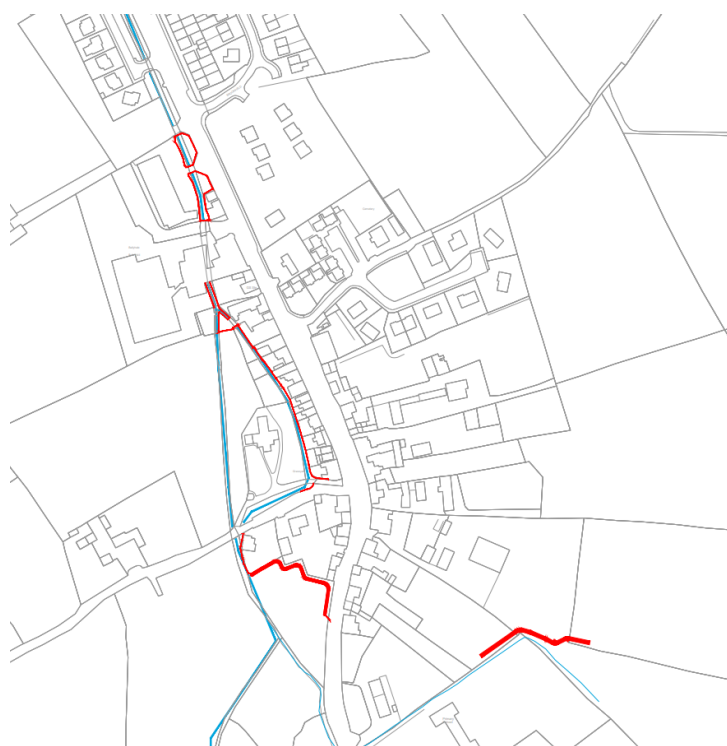
Figure 4-3: Concept Hard Defences Required
